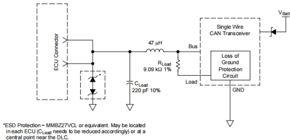
Figure 7. Single Wire CAN Network
